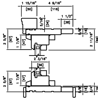
WOOD EXTERIOR DOUBLE 4 9/16" (116mm) 2" BRICKMOULD
