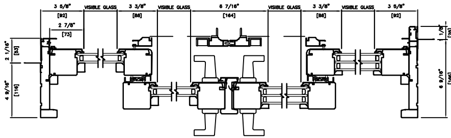
METAL CLAD DOUBLE/DOUBLE/TRIPLE/TRIPLE FOUR PANEL 4 9/16" (116mm)/6 9/16" (166mm)
